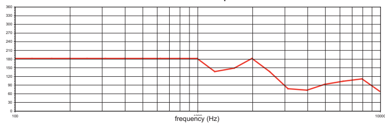
Horizontal off-axis response
