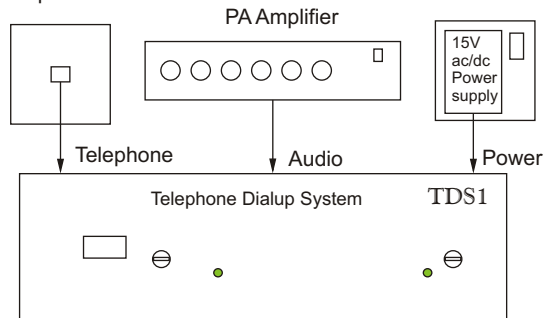
Telephone Socket
